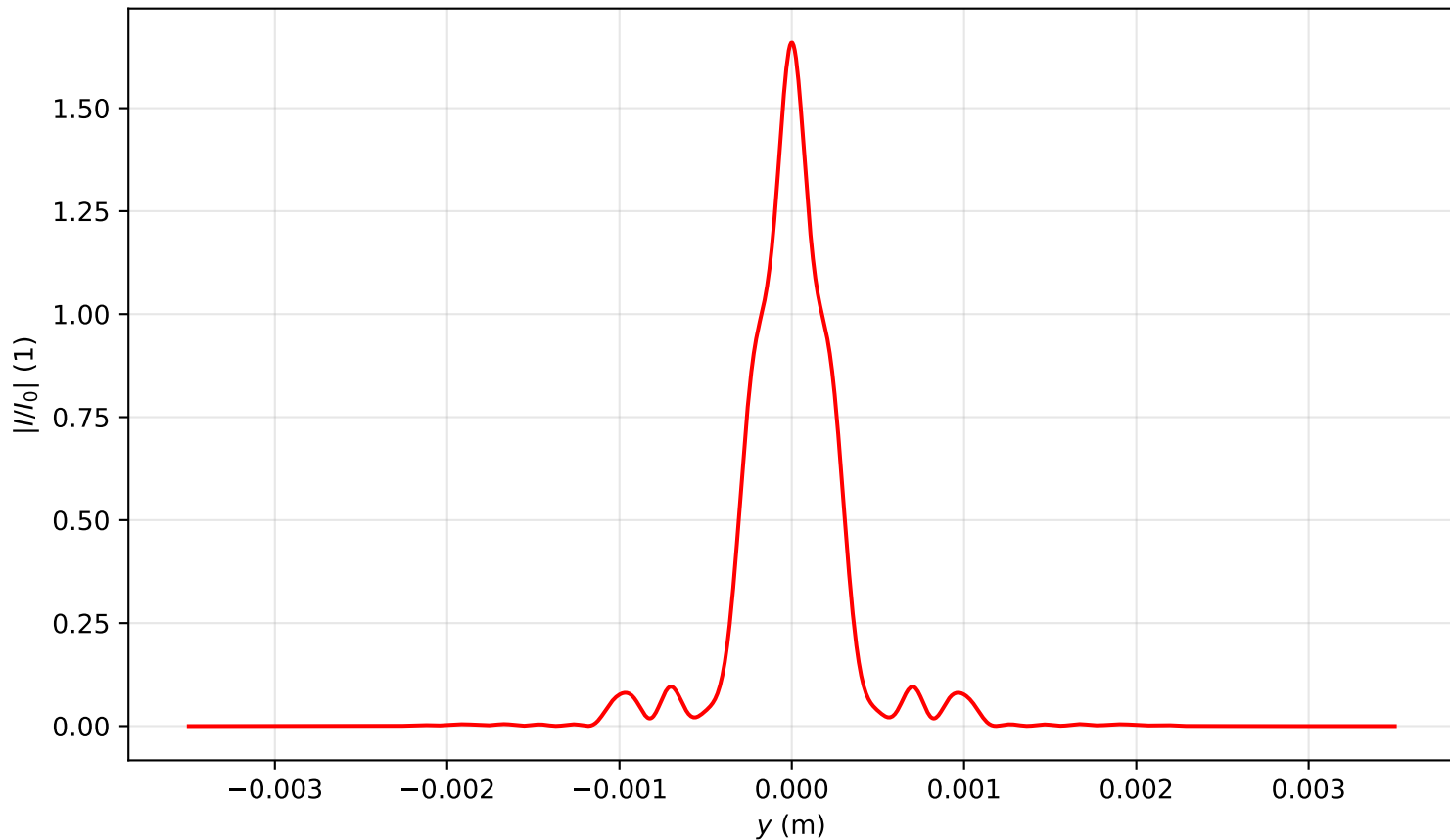
Intensity profile I(x=0, y, z=1.194)/I_0 , P_{in}=6.5P_{cr} , artificial time
